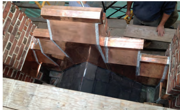
Copper Sheet Metal Coping Cap
